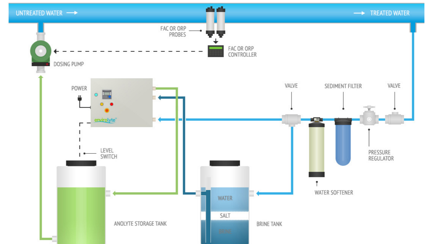
Typical layout of Envirollyte water disinfection system
